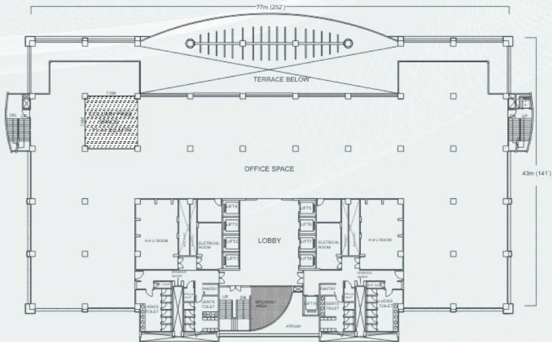
6TH AND 10TH FLOOR PLAN
